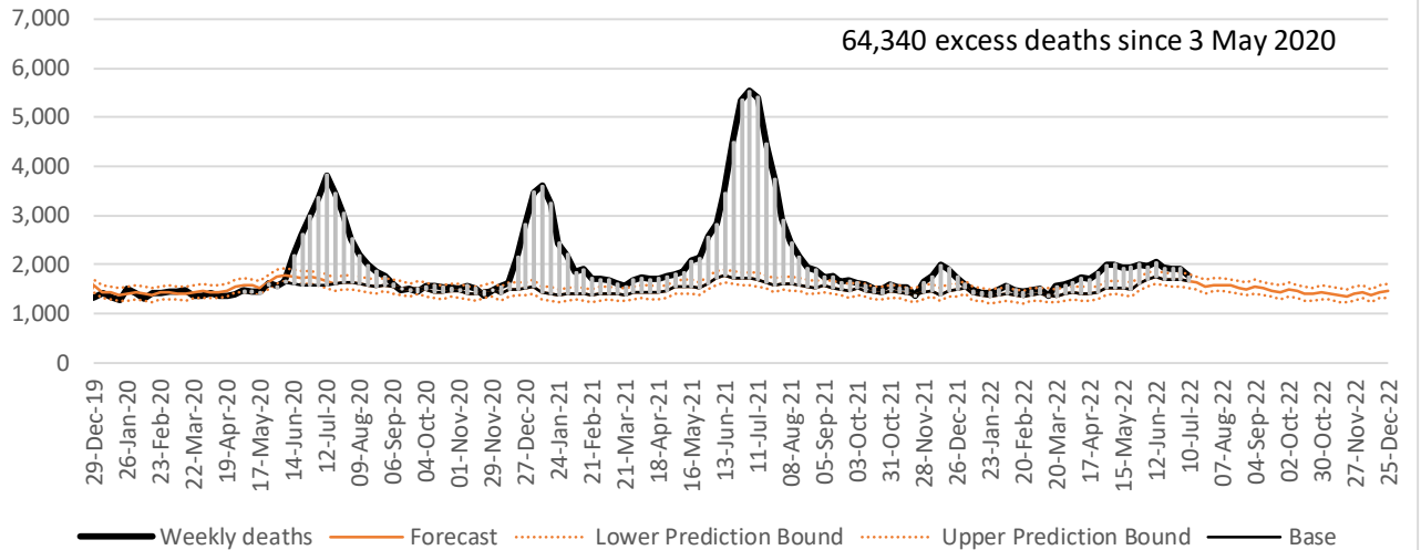
Gauteng weekly deaths from natural causes : 29 Dec 2019 - 16 Jul 2022
