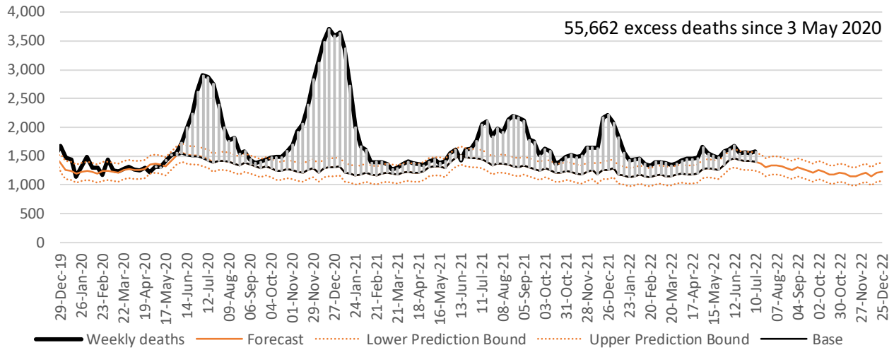
Eastern Cape weekly deaths from natural causes : 29 Dec 2019 - 16 Jul 2022
