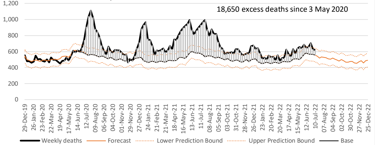
Free State weekly deaths from natural causes : 29 Dec 2019 - 16 Jul 2022
